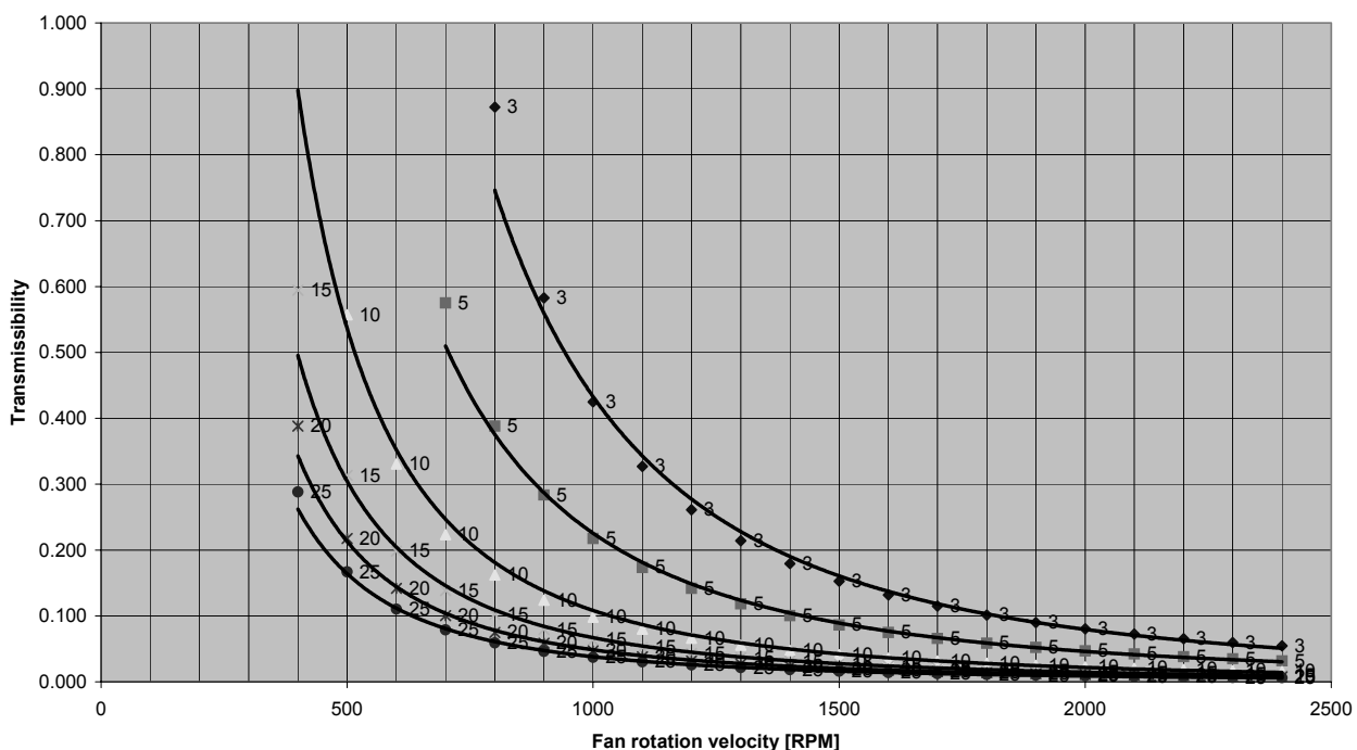
Transmissibility
